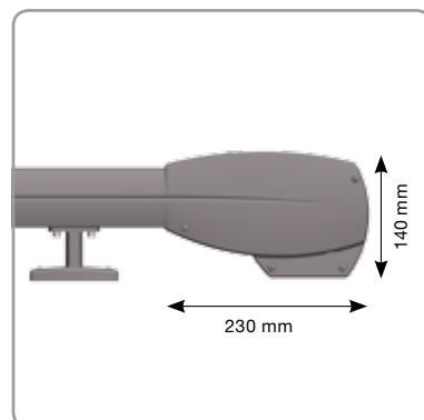
Dimensions caisson
